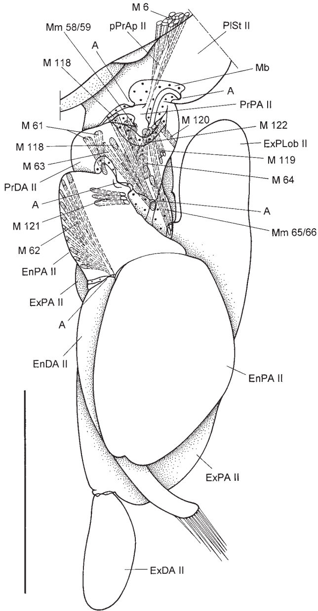
Fig. 9. Metaphreatoicus australis , ♂, right pleopod II in posterior view. – Scale: 1 mm.
