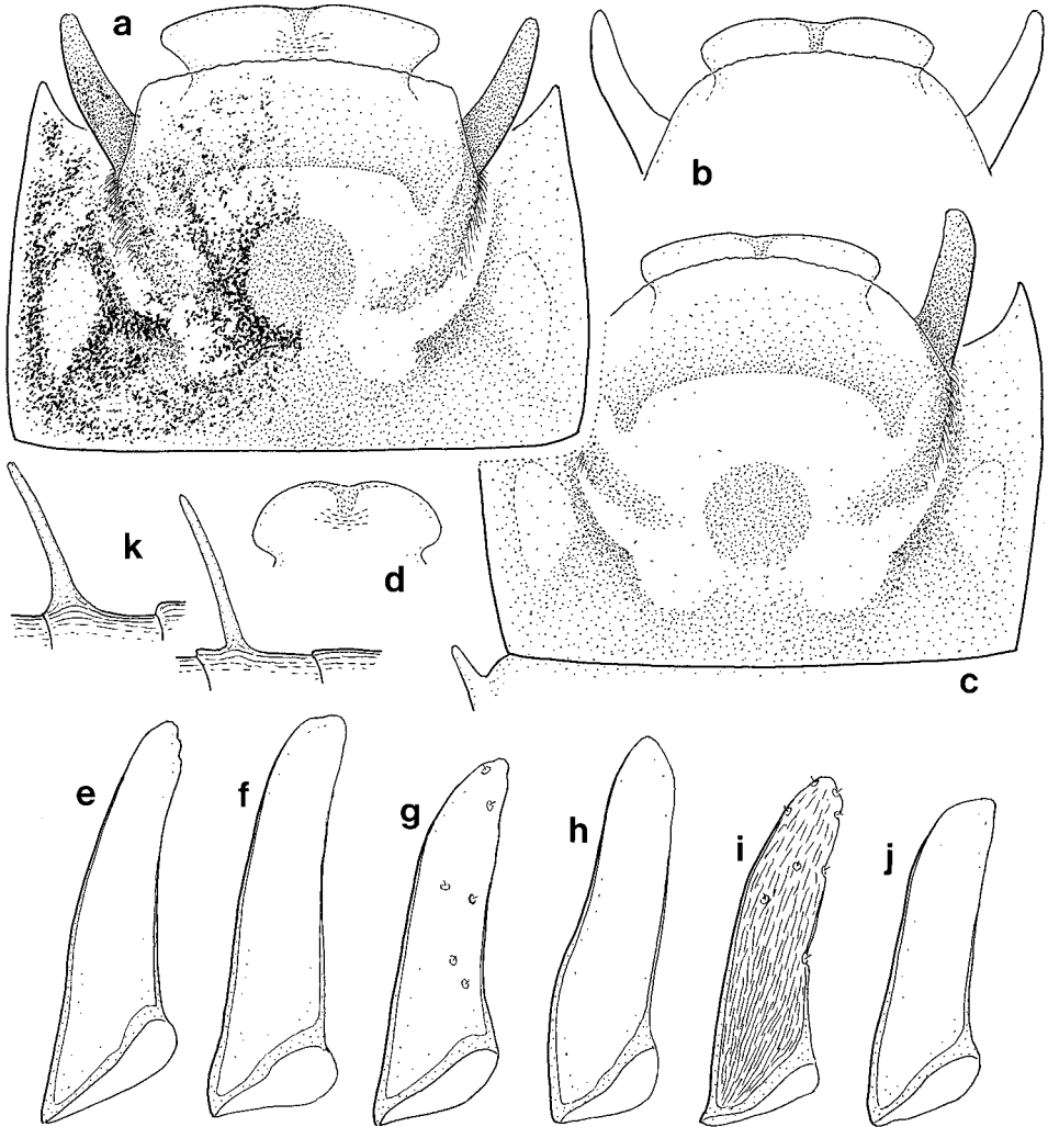
Fig. 3. Caenis ludicra Navas; male. – a, b and d. Genitalia: specimens from Tucuman, different shapes of penis and styliger-plate; – c. genitalia from a specimen from Alta Gracia (MZB); – e–j. variability of forceps-shape: g with sensillae, i with trichoma and sensillae; – k. fingerlike process on the second abdominal tergite.
