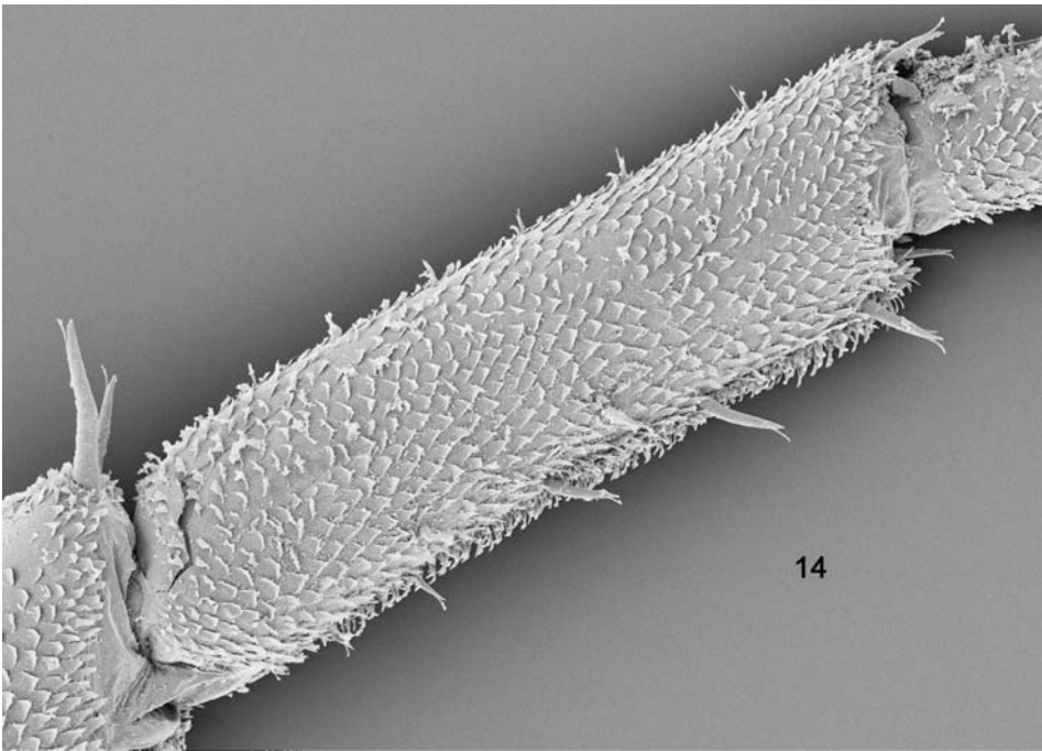
Figs. 13–14. Utopioniscus kuehni n. sp., paratype ♂, 12 mm long, Grotta della Utopia (SMNS T567), SEM-photographs after critical point treatment. – 13. Pereiopod I. 14. Carpus of pereiopod I. – Scale: 0.5 mm.
