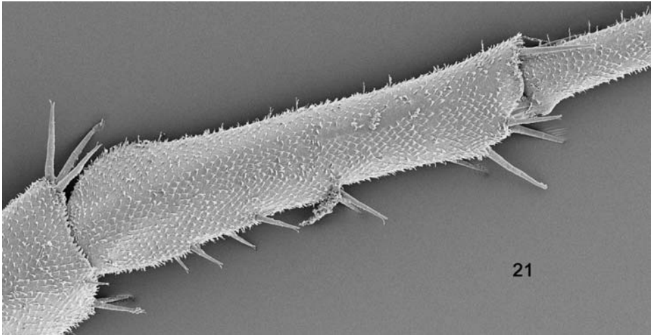
Figs. 19–21. Utopioniscus kuehni n. sp., paratype ♂, 12 mm long, Grotta della Utopia (SMNS T567), SEM-photographs after critical point treatment. – 19. Pereiopod VII. 20. Ischium and merus of pereiopod VII. 21. Carpus of pereiopod VII. – Scale: 1 mm.
