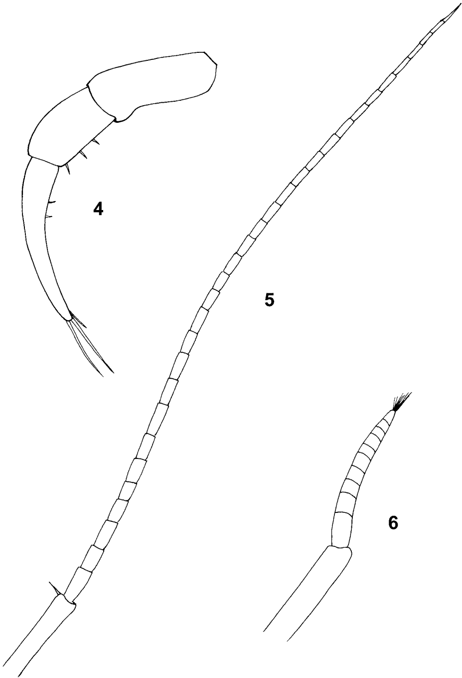
Figs. 4-6. Antennal flagellum and antennula. - 4-5. Utopioniscus kuehni n. sp., holotype ♀. 4. Antennula. 5. Flagellum of antenna. - 6. Cantabroniscus primitivus , flagellum of antenna, after VANDEL (1965b: 492).
